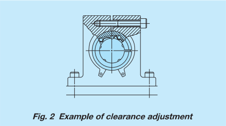
Fig. 2 Example of clearance adjustment
