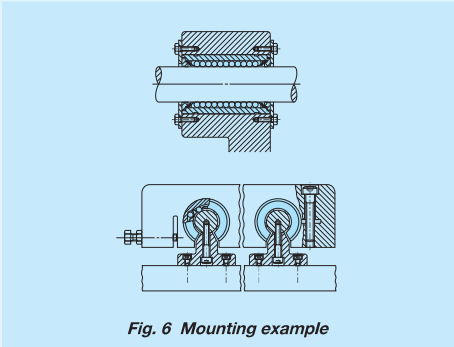
Fig. 6 Mounting example
