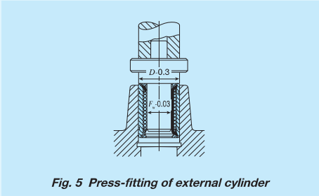
Fig. 5 Press-fitting of external cylinder
